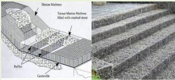
Fig. 3: Gabion mattress
