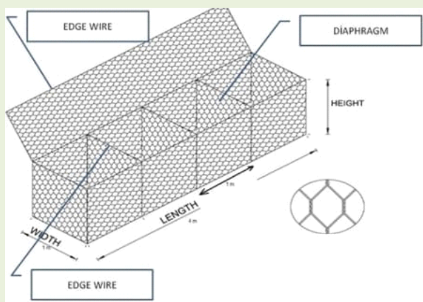
Fig. 1: Wire mesh boxes for gabions
